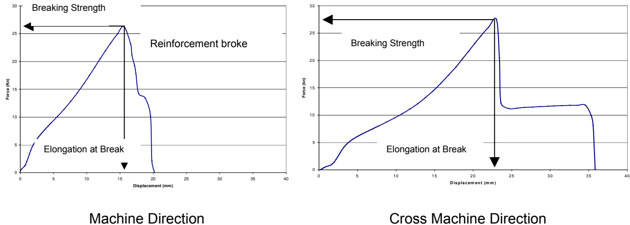
Figure 1 Typical Force displacement curve for tensile test of polyester reinforced roof membrane (Sample 21C) in the machine (MD) and cross directions (CD)
